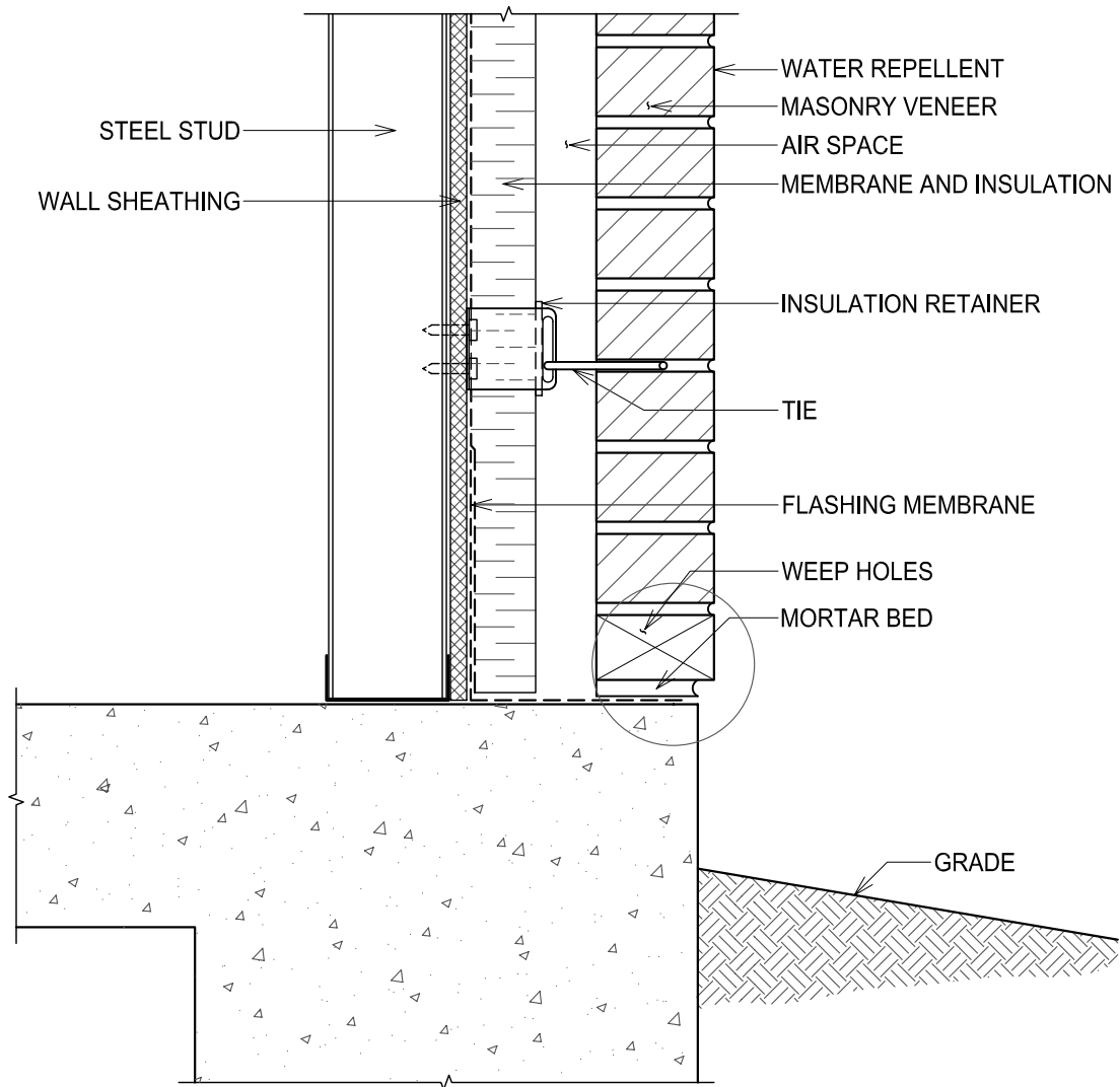
VENEER DETAILS - STEEL STUD BACKUP AT BASE - CONCRETE SUPPORT - DETAIL S1.1
