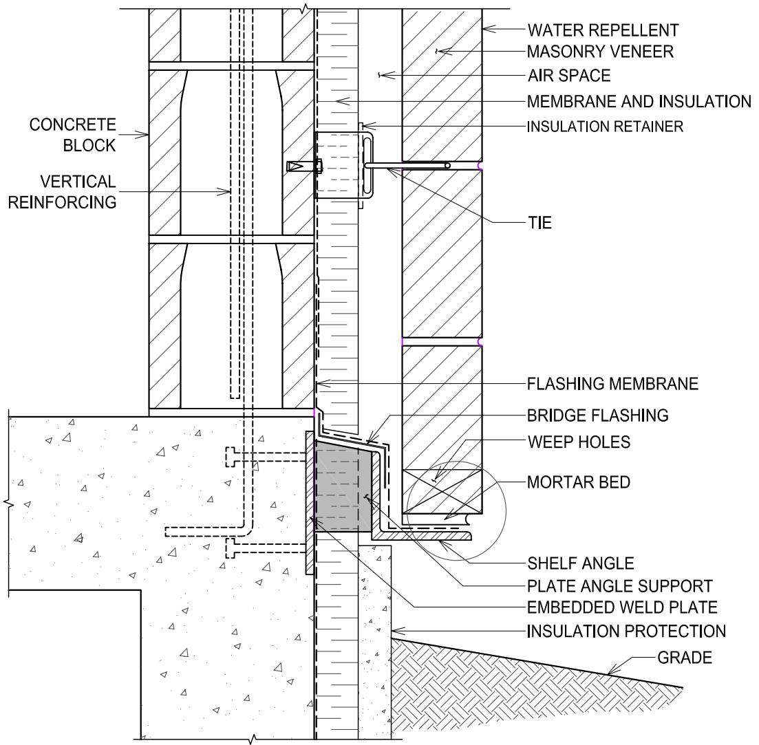
VENEER DETAILS - BLOCK BACKUP AT BASE - SHELF ANGLE SUPPORT - DETAIL 2
