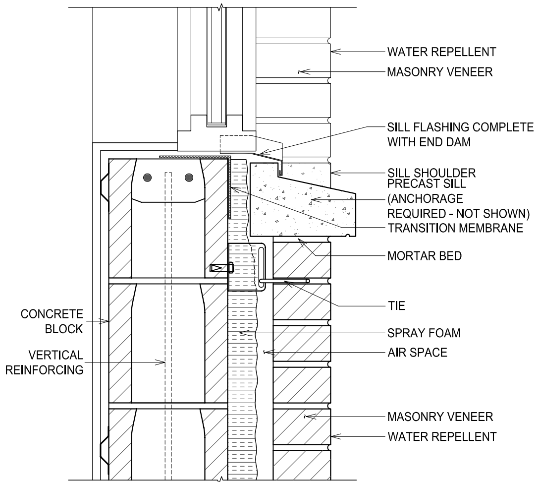
VENEER DETAILS - BLOCK BACKUP AT WINDOW SILL - PRECAST CONCRETE SILL - DETAIL 4
