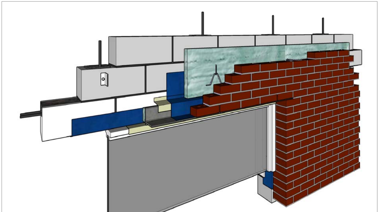
VENEER DETAILS - BLOCK BACKUP AT WINDOW HEAD - LINTEL SUPPORT - DETAIL 6
