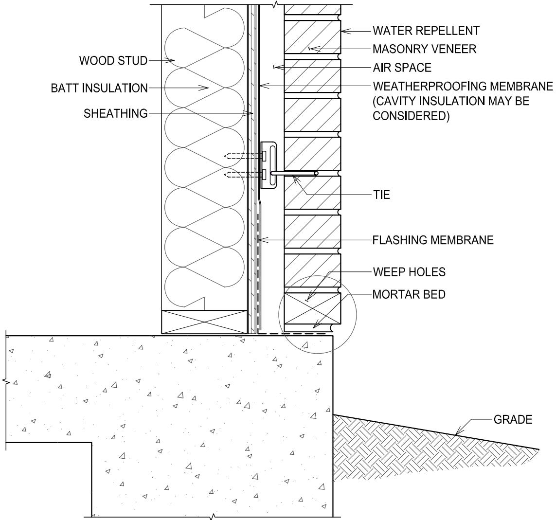
VENEER DETAILS - WOOD STUD BACKUP AT BASE - CONCRETE SUPPORT - DETAIL 15
